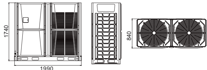
Fig. 3.6 Shape6 (26HP~32HP)
