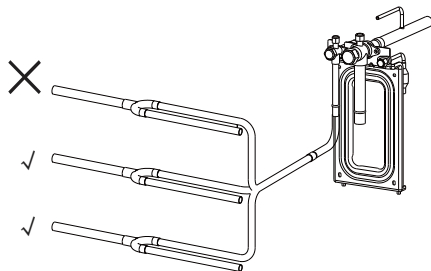
Fig. 4.11 Installation 1
