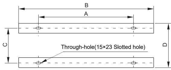
Fig. 3.8 bolts location
