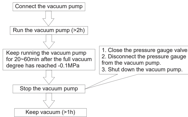
Fig. 4.5 Vacuumizing
