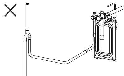
Fig. 4.12 Installation 2
