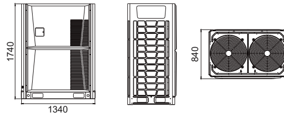
Fig. 3.4 Shape4 (22HP)
