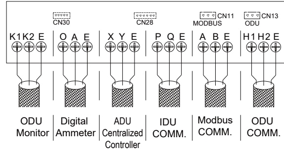
Fig. 5.2 Communication terminal
