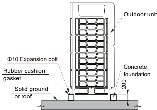
Fig. 3.7 Foundation
